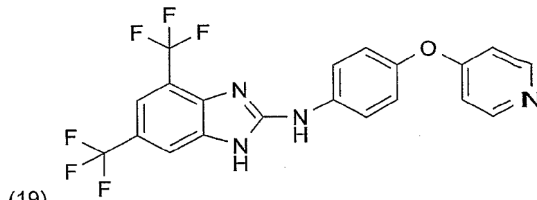
(19) (4,6-Bis-trifluoromethyl-1H-benzimidazol-2-yl)-[4-(pyridin-4-yloxy)-phenyl]-amin
